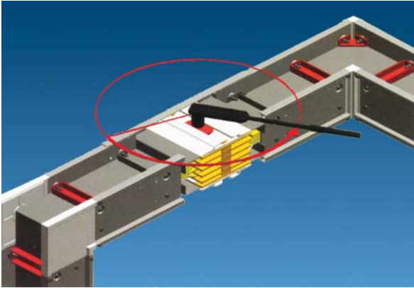
HCC-XLC 密集型母线槽 HCC-XLC Intensive bus groove
