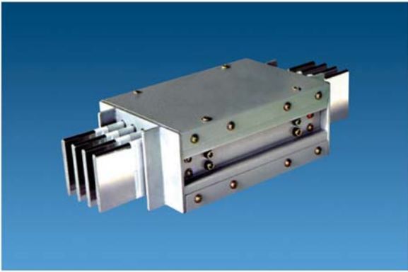
HCC-FLD 风力发电母线槽 HCC-FLD Wind Power Busbar
